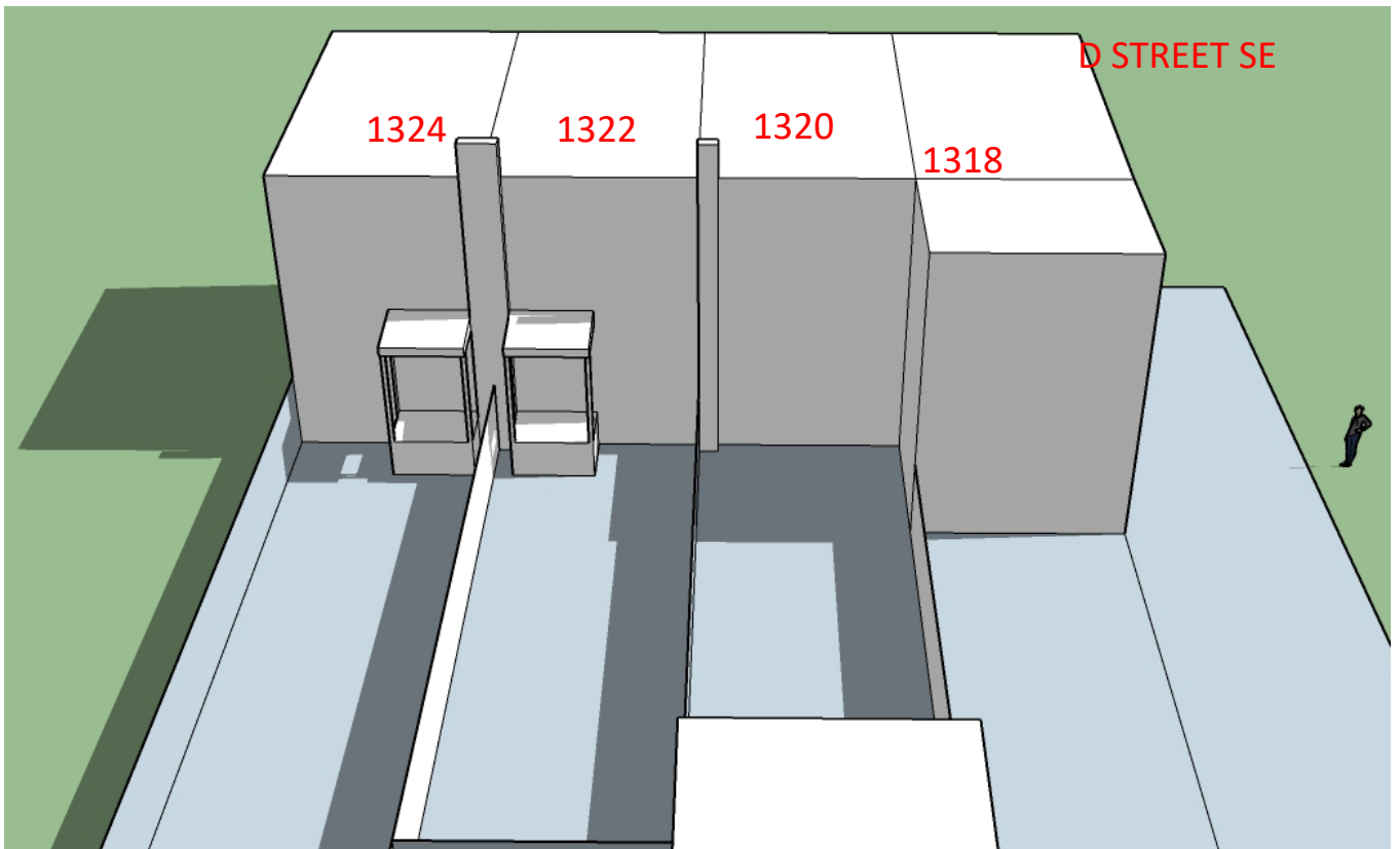
June 21 st 3:30 PM TWO STORY OPTION- 13' DEEP
