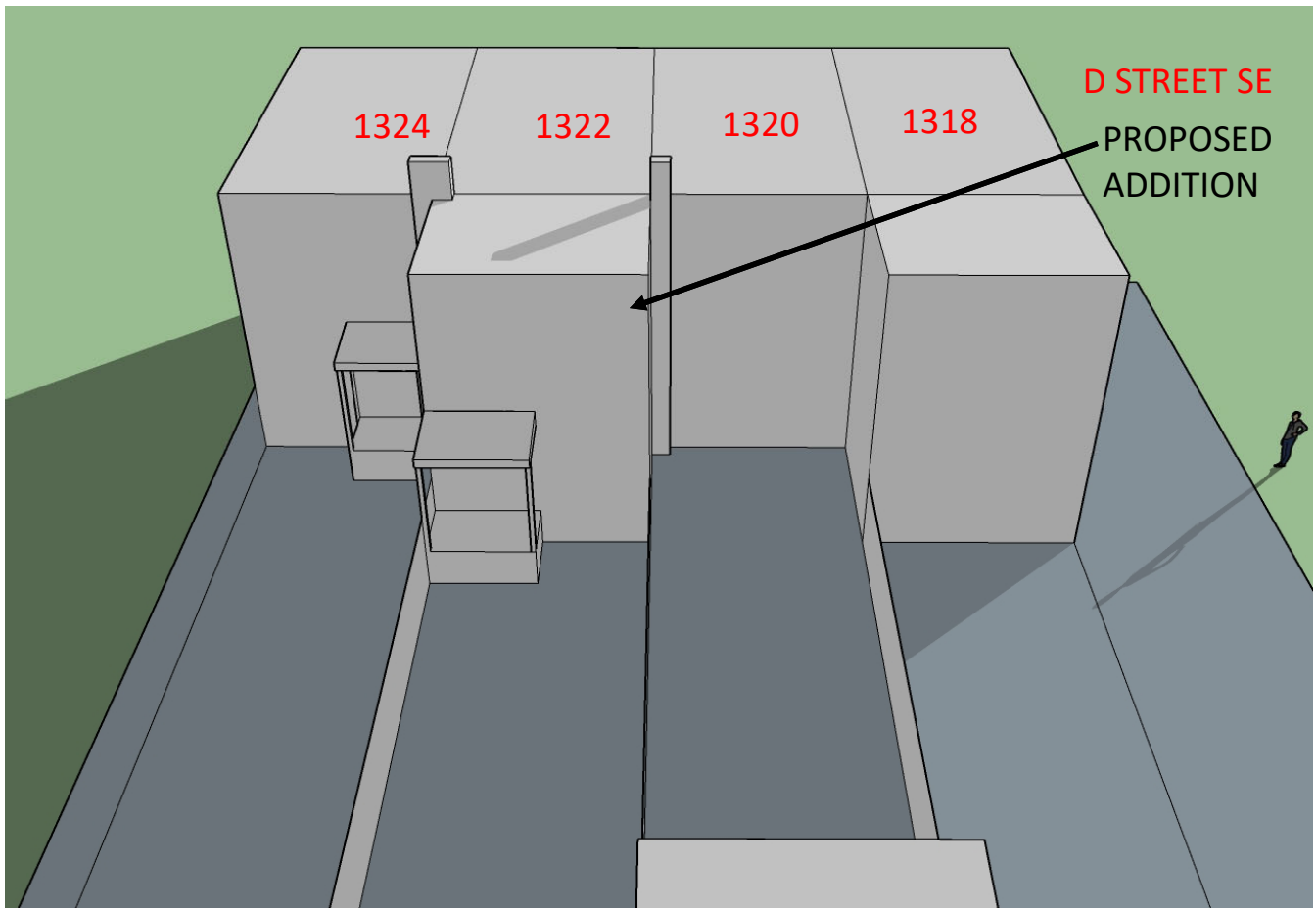
December 21 st 3:30 PM TWO STORY OPTION- 13' DEEP
